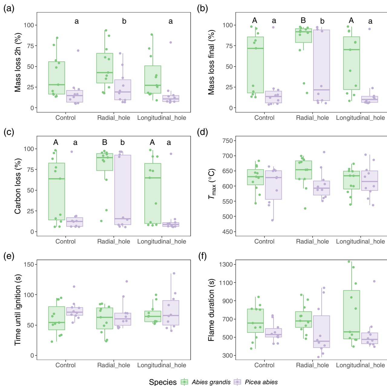
FIGURE 1 Boxplot showing the distribution of flammability parameters of two gymnosperm species under three experimental treatments. Dots are raw data. Mass loss 2 h represents percentage mass loss after 2 h (in percentage), mass loss final represents final percentage mass loss (in percentage), and T_{max} represents mean maximum temperature (in degrees Celsius). Different uppercase letters indicate significantly different effects of treatments on Abies grandis , and lowercase letters on Picea abies , as revealed by linear mixed model results (see Appendix S1: Table S2), followed by a post hoc test ( p < 0.05 ; see Appendix S1: Table S3). The absence of lowercase and uppercase letters denotes no significant influences.
