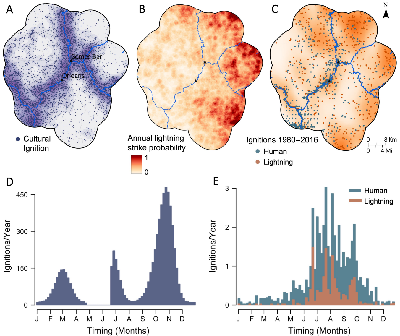
FIGURE 5 Spatial and temporal distribution of annual cultural ignitions on the Somes Bar landscape (A, D), contemporary lightning strike patterns (B), and contemporary ignition patterns (C, E). Maps depict cultural ignitions from one simulated year (A), annual lightning strike probability within a 2 km window (B), and human and lightning ignition locations and interpolated density recorded between 1980 and 2016 from Short (2017; C). Graphs display cultural ignition timing averaged more than 200 simulated years (D) and a stacked bar chart of ignition timings for all ignitions recorded on the Somes Bar landscape from 1980 to 2016 with lightning in orange and human ignitions in blue (E).
